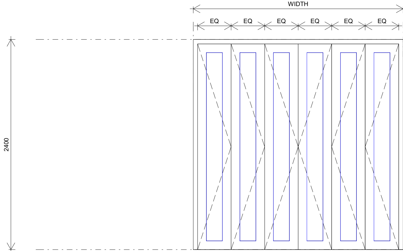
D09 - GLAZED BIFOLD DOOR 1:25
